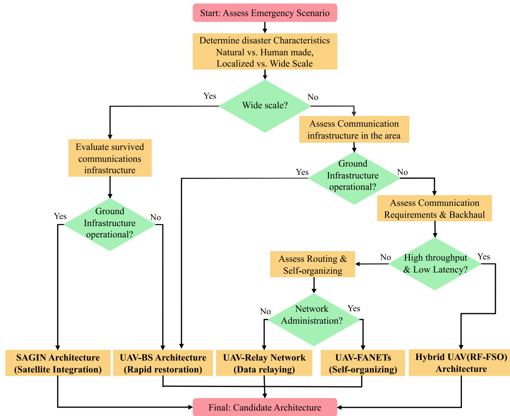
Fig. 8. Architecture selection flowchart for UAV-assisted emergency communications as a function of incident scale, residual infrastructure, latency/throughput targets, and energy budget.
