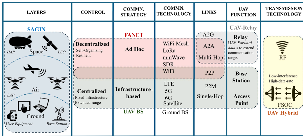
Fig. 7. Decision criteria distinguishing UAV emergency architectures (primary UAV role, hop count/topology, coordination mode, link heterogeneity) and expected overlaps; the hybrid qualifier is cross-cutting.
