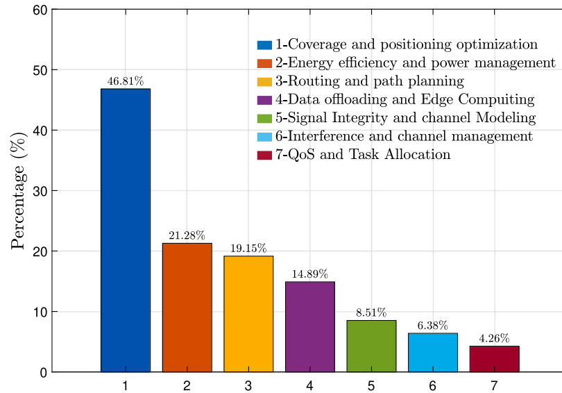
Fig. 13. Distribution of optimization methodology categories applied in UAV emergency communications. Note: Percentages can exceed 100% because many studies target multiple categories.
