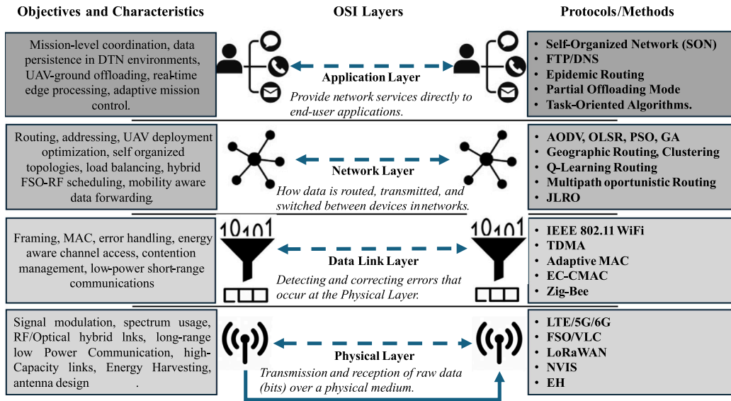
Fig. 5. Observed protocol stack in UAV emergency networks: mapping to OSI layers and indicative data flow.
