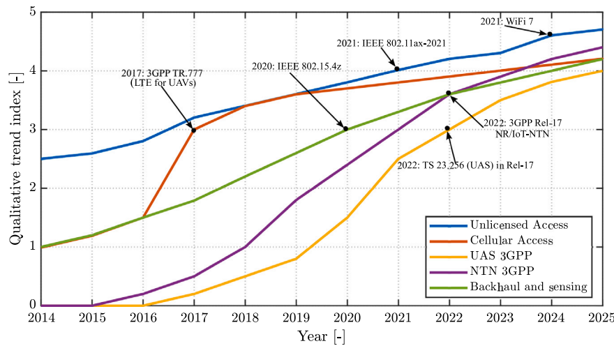
Fig. 1. Evolution of UAV-enabling wireless technologies since 2014. The 0–5 “maturity and attention” index is an ordinal, qualitative trend indicator.
